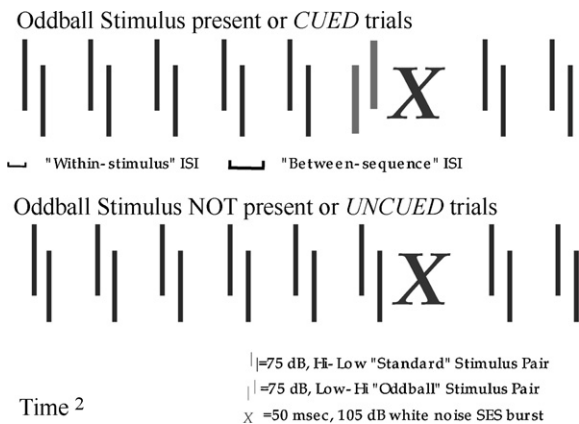
Fig. 2. Sample two-tone sequence trials (cued and uncued). Comparable results are obtained when the background stimulus is lo-hi, and the oddball is hi-lo (unpublished data); adapted from Ref. [6].
