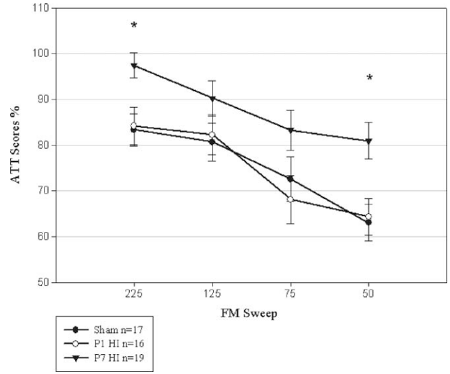
Fig. 8. Means ( \pm S.E.M.) for attenuation response scores (ATT scores) on the variable duration FM sweep procedure in adulthood for P1/P7 HI and shams animals. P7 HI animals showed a main effect for treatment in comparison to sham animals, indicating impaired performance on this complex task. P7 HI animals * p<.01 , comparison between P7 HI and sham groups.
