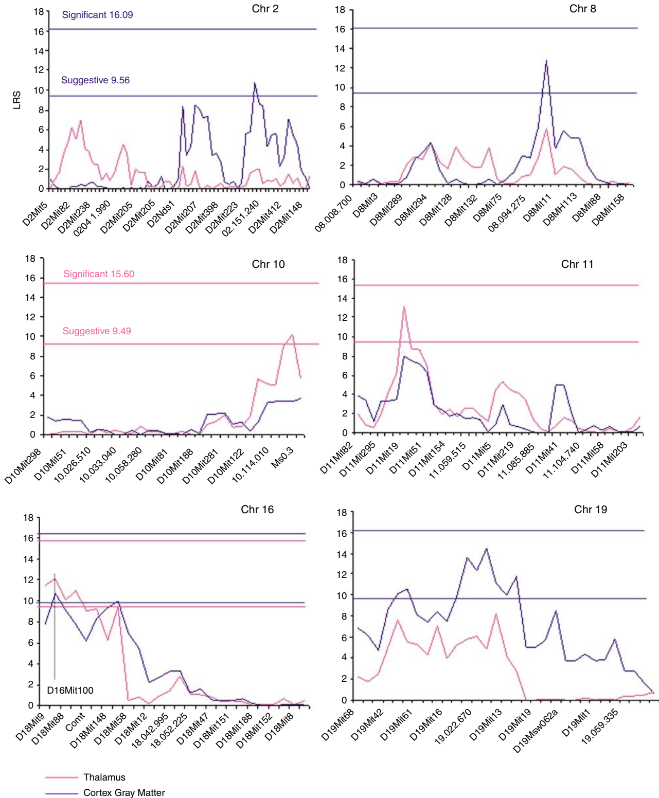
Figure 3 LRS scores for structural measures. Pink lines illustrate the LRS scores for uncorrected thalamus volumes. Three QTLs were identified on chromosomes 10, 11 and 16. Blue lines illustrate the LRS scores for cortex gray matter volume strain means adjusted for age. Four QTLs were identified on chromosomes 2, 8, 16 and 19. The Y axis represents the LRS scores as determined by marker regression at each microsatellite marker along the X axis. LRS\ score = 1/4.6 the logarithm of the odds ratio (the LOD score). The data are presented as LRS plots with lines connecting the intervals between the LRS data points. A single QTL (peak at D16Mit100 , indicated by the dotted black line in panel 5) on chromosome 16, was associated with both thalamus and cortex gray matter volumes.
