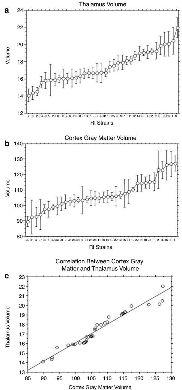
Figure 2 Interaction line plots summarizing the variability of structural volumes across RI strains (means and standard deviation) (see (a) for thalamus volumes and (b) for cortex gray matter volumes). Strains are ordered by feature volume. Panel c represents the correlation between the two volume measures across the strain means.
